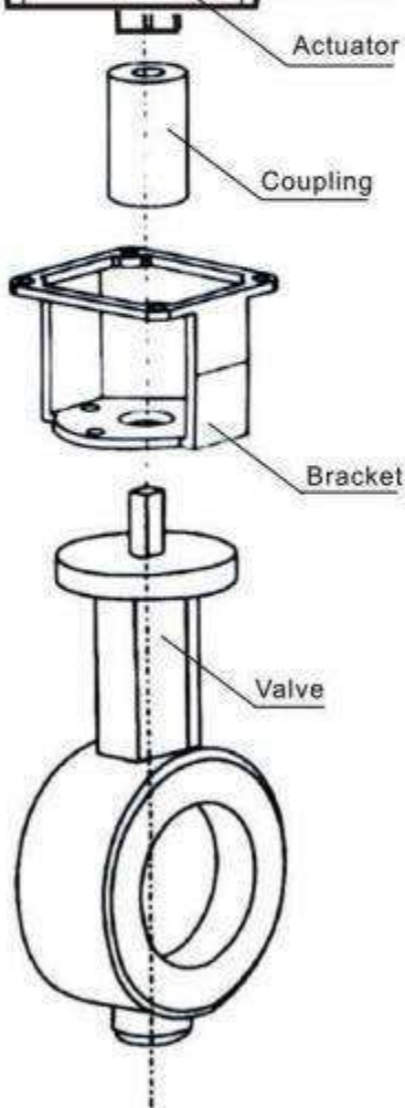
Assembly Drawing
