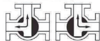
L-Pattern Flow Direction Diagram
